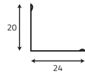
Wall Angle
