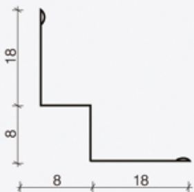
WALL ANGLE (W)
