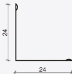
WALL ANGLE 24/24 (L)
