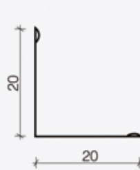
WALL ANGLE 20/20 (L)
