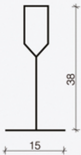
MAIN TEE 15/38 ( T-15)
